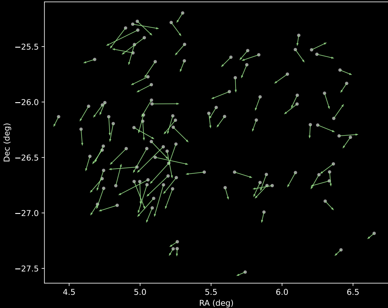
APOGEE DR17 Cluster 5 Proper Motion Vectors (n=104)
