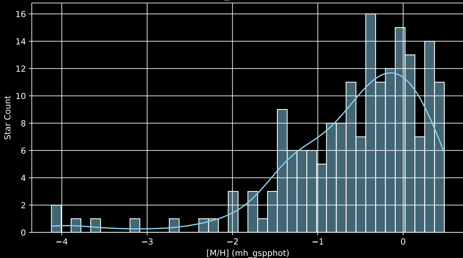
APOGEE DR17 Field: [002+02-O [M/H] (mh_gspphot) (n= 183)
