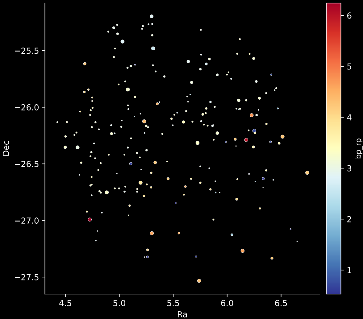
APOGEE DR17 Field: [002+02-O] Stars: 205
