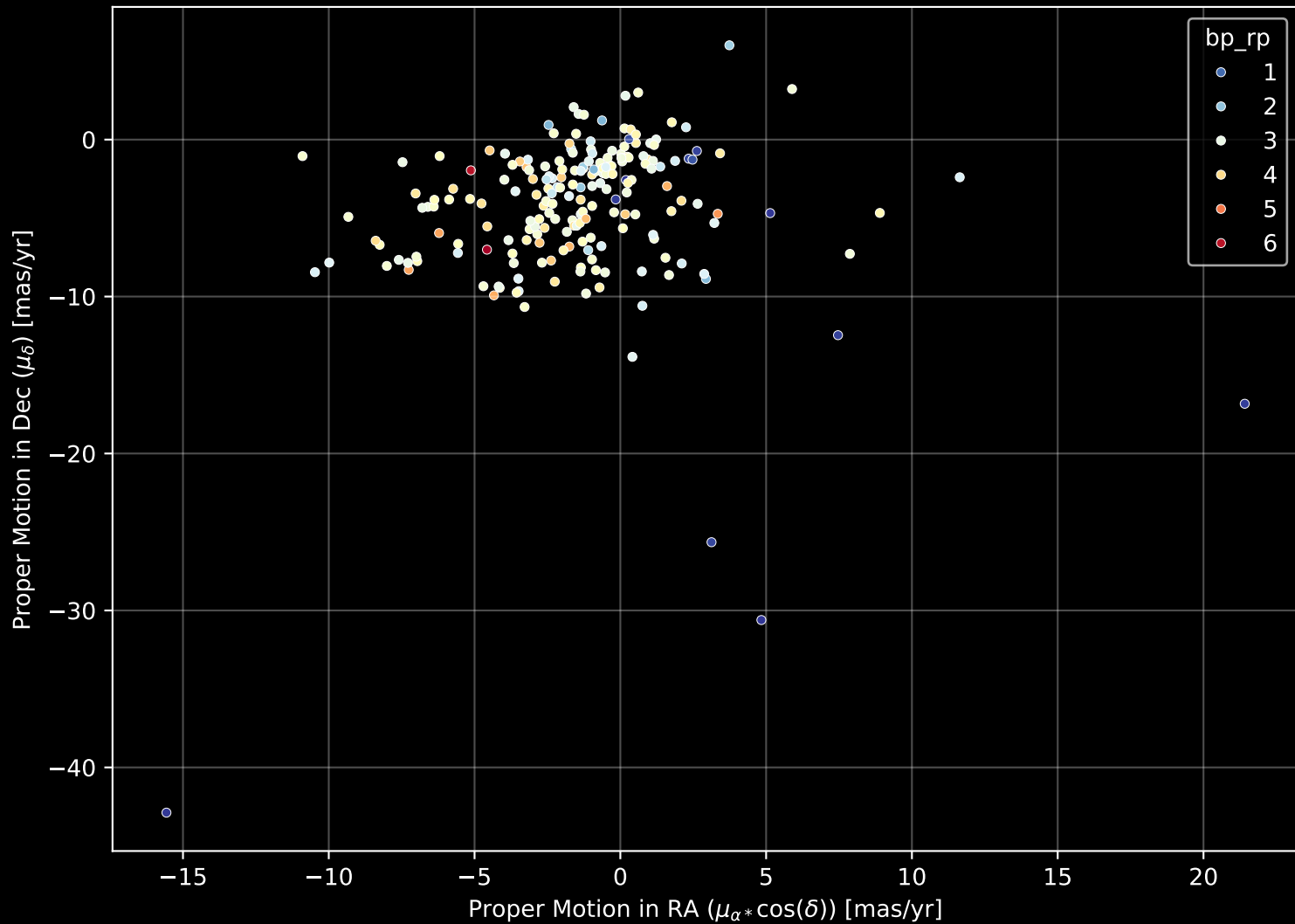
APOGEE DR17 Field: [002+02-O] Proper Motion Diagram (n= 205)
