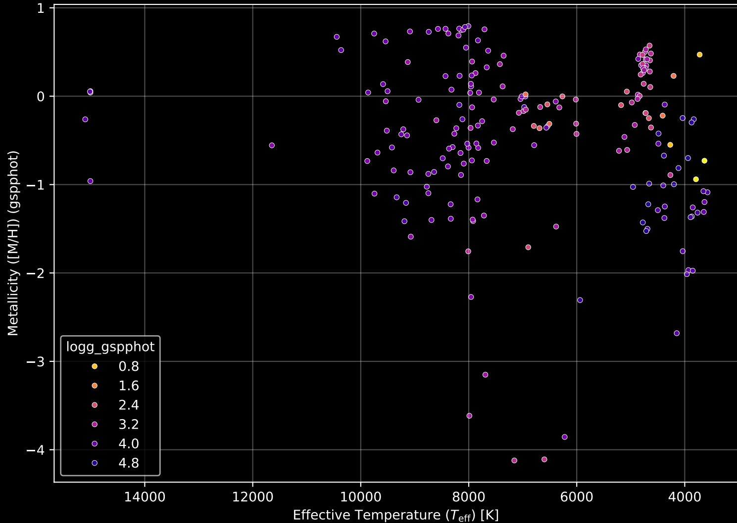
APOGEE DR17 Field: [002+02-O] Stellar Population Parameters (n= 205)
