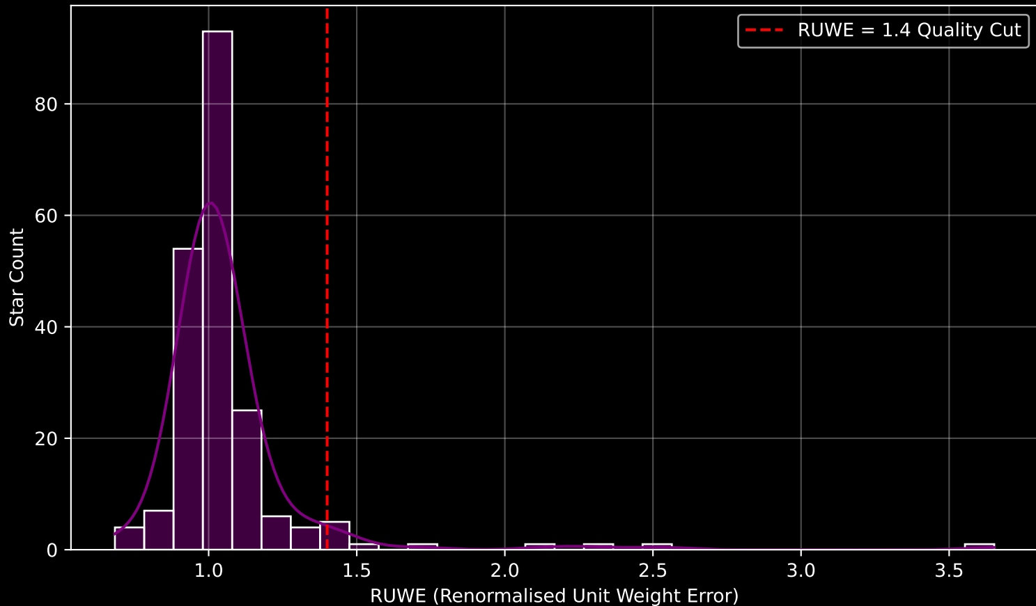
GAPOGEE DR17 Field [002+02-O] RUWE Distribution (n= 204)
