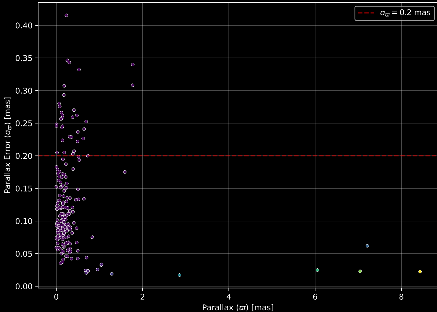
APOGEE DR17 Field: [002+02-O] Parallax Quality (n= 205)
